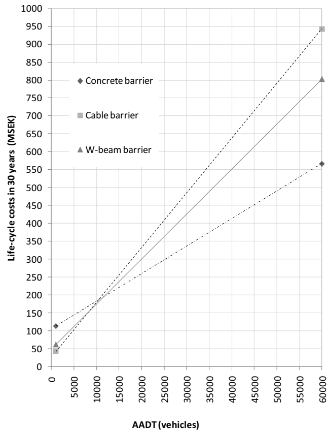
Figure 6.5 Effect of AADT on life-cycle costs for the studied barrier types
